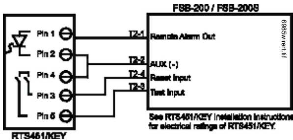
Wiring Diagram with RTS451/KEY
