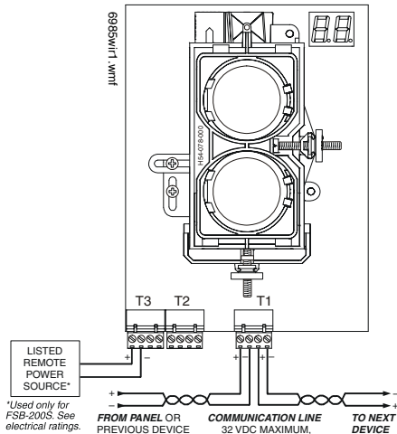
Wiring Diagram
